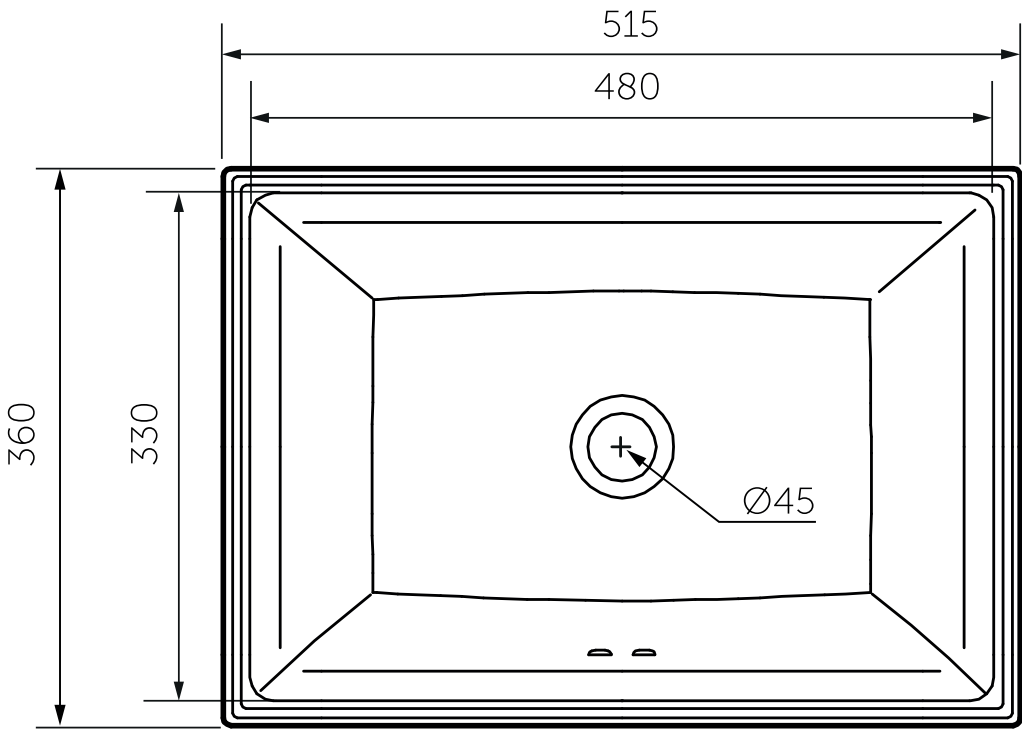
VISTA SUPERIOR / TOP VIEW
