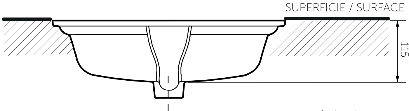
VISTA FRONTAL / FRONT VIEW
