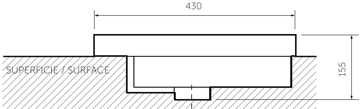
VISTA LATERAL / LATERAL VIEW
