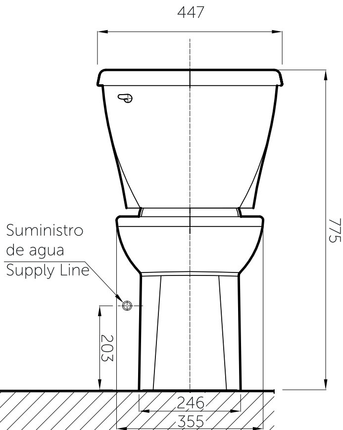
VISTA FRONTAL / FRONT VIEW
