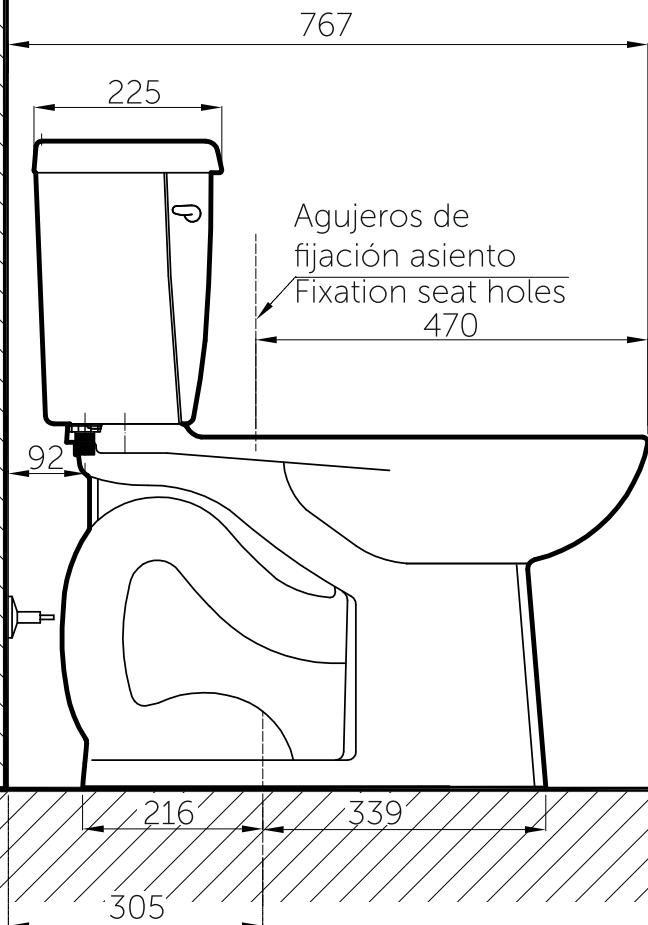
VISTA LATERAL / LATERAL VIEW
