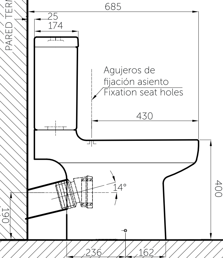
VISTA LATERAL / LATERAL VIEW
