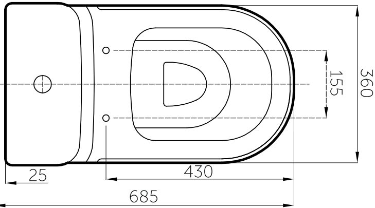
VISTA SUPERIOR / TOP VIEW
